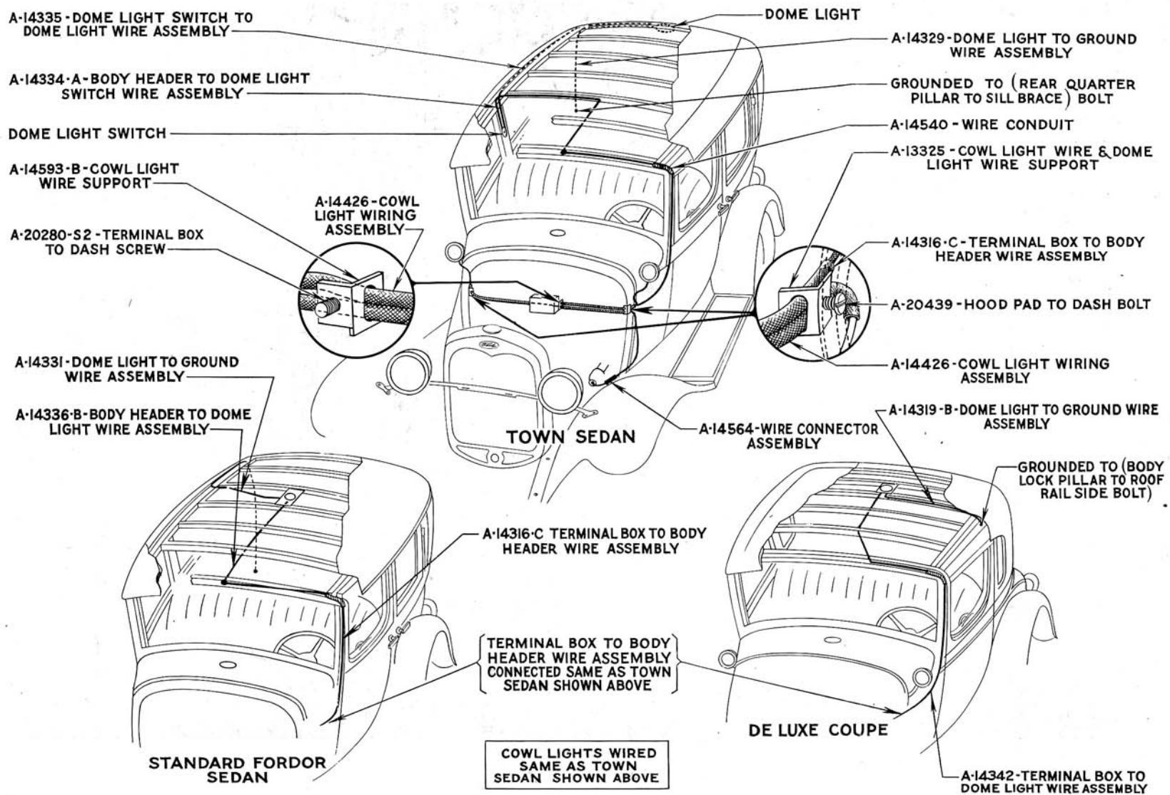
Fig. 938—Wiring Diagram of Town Sedan, Standard Fordor Sedan and DeLuxe Coupe
